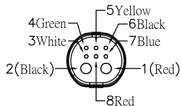
WPB25-26M 2+6
