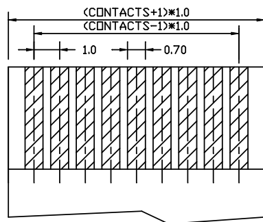
FFC/FPC DIMENSION THICKNESS 0.30 mm
