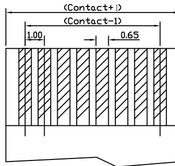
FFC/FPC DIMENSION THICKNESS 0.30 mm
