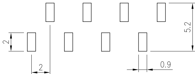
PCB Layout
